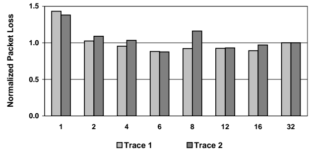
Figure 8: Normalized Packet Loss when Moving or Promoting Different Numbers of Hash Buckets
