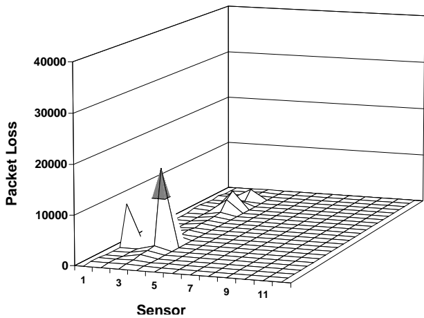
Figure 5: Number of Packets Dropped per Sensor over Time with Dynamic Feedback
