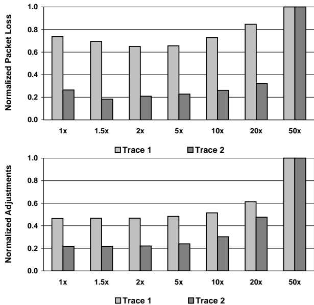
Figure 11: Loadbalancer Performance when Changing the Threshold to Promote Hash Buckets
