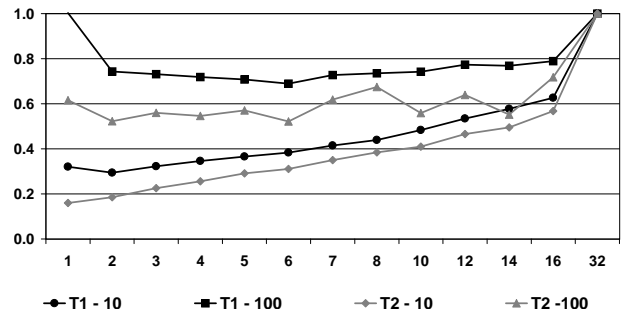
Figure 10: Loadbalancer Performance Tradeoff when Adjusting Different Numbers of Hash Buckets
